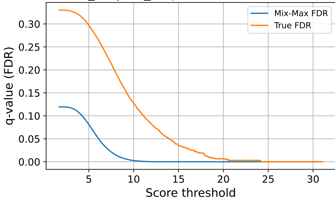
flows_24 | val_target — FDR vs Threshold
