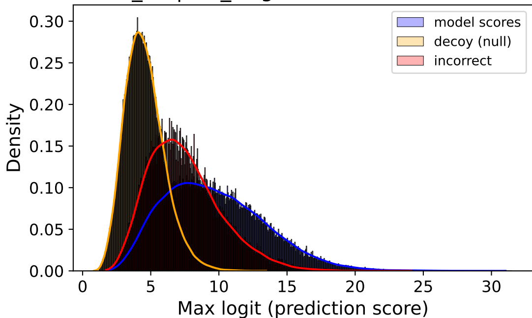
flows_24 | val_target — Score Distributions
