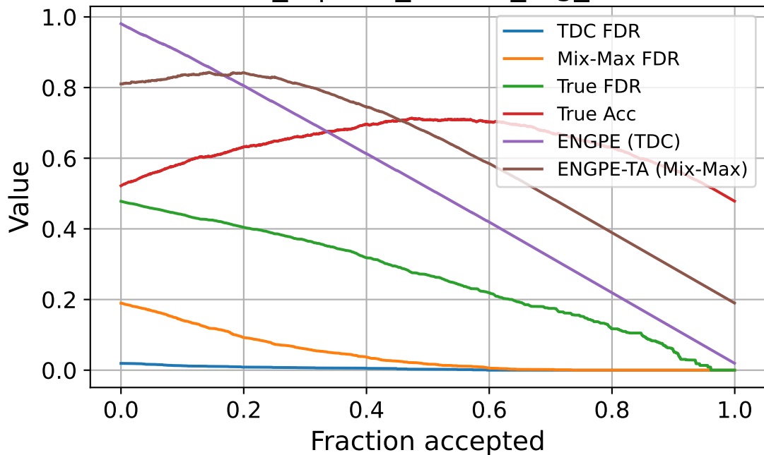
flows_6 | corr_source_fog_sev5
