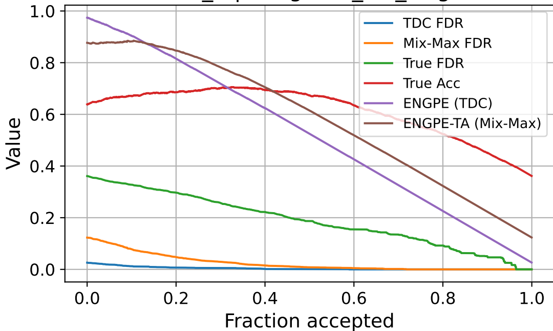
flows_6 | imagenet_val_target
