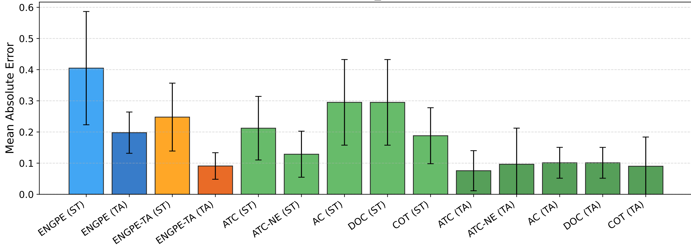
BREEDS nonliving26 [flows_6] — MAE [corruptions]
