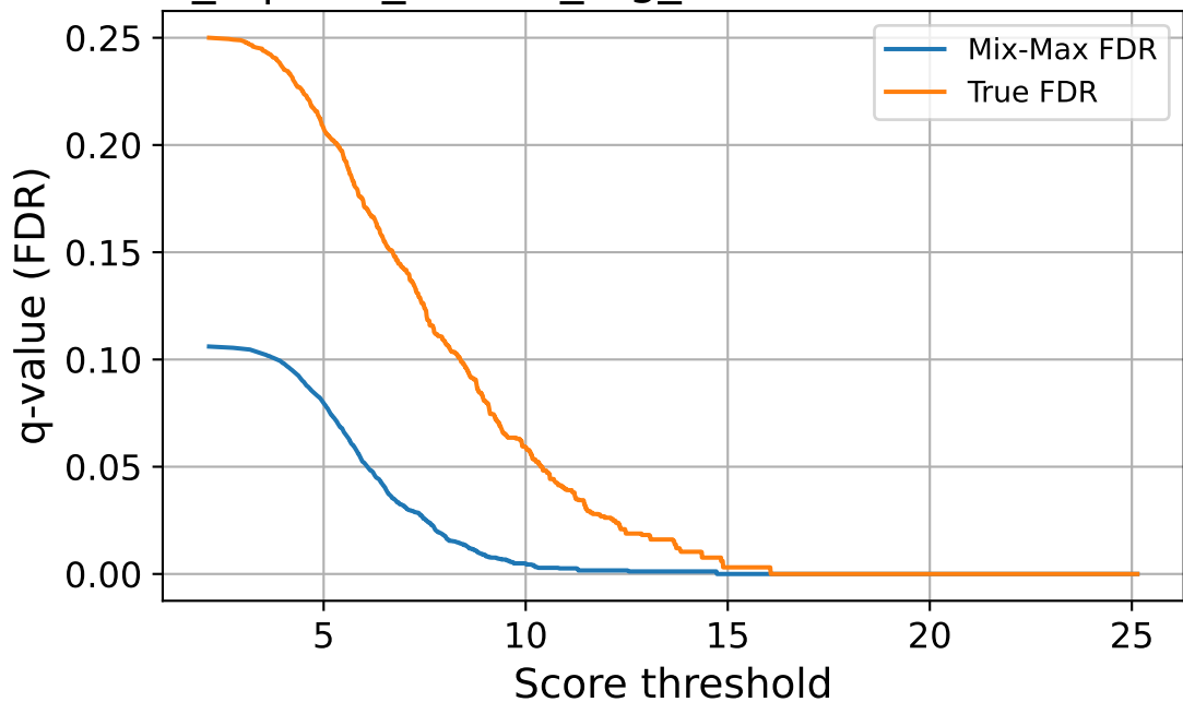
flows_6 | corr_source_fog_sev3 — FDR vs Threshold
