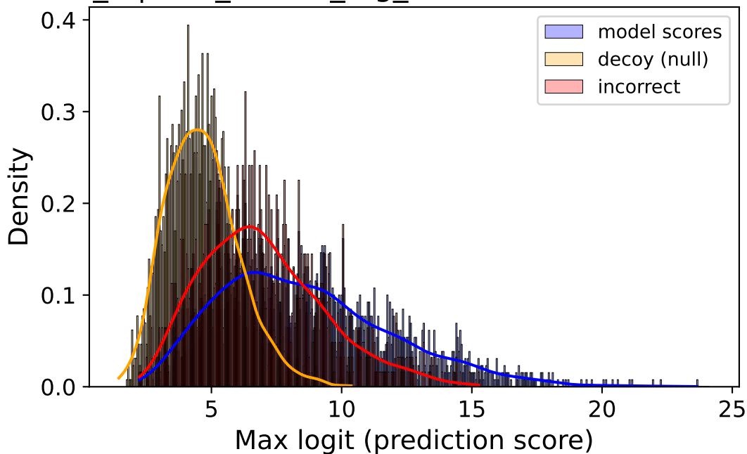
flows_6 | corr_source_fog_sev5 — Score Distribution
