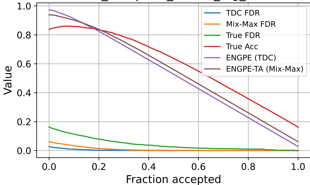
seed_123 | corr_source_fog_sev2
