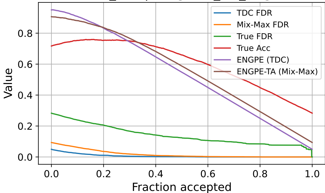
seed_123 | imagenet_val_target
