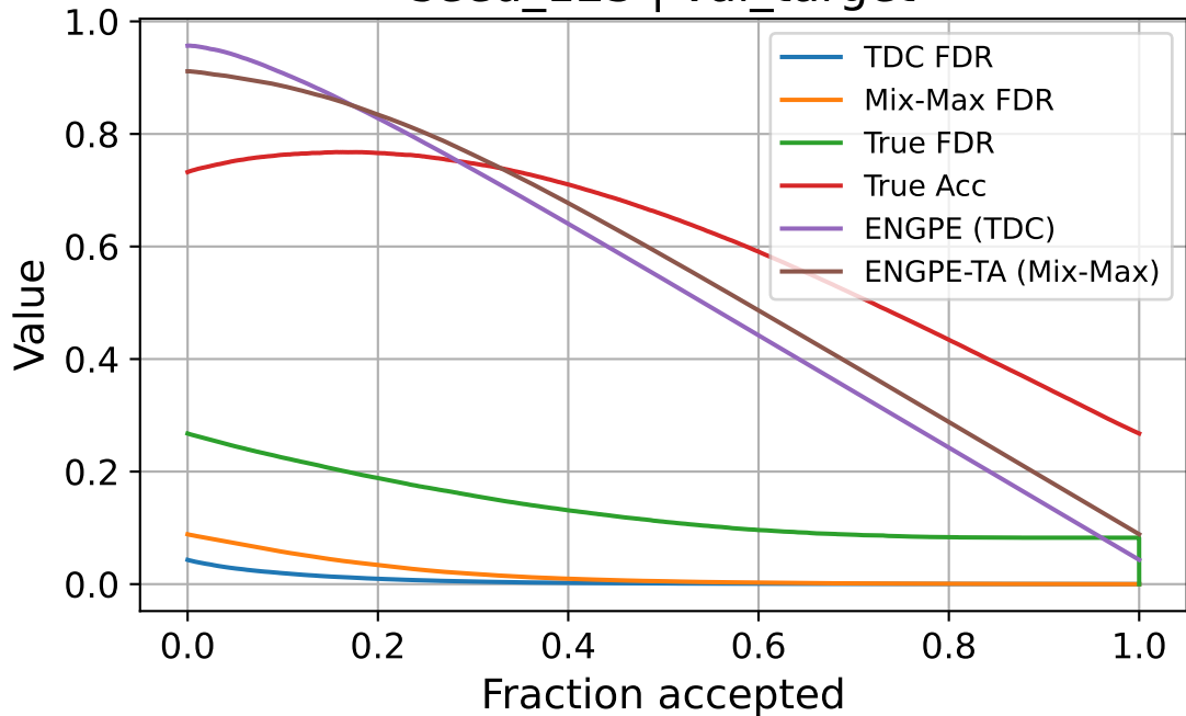
seed_123 | val_target
