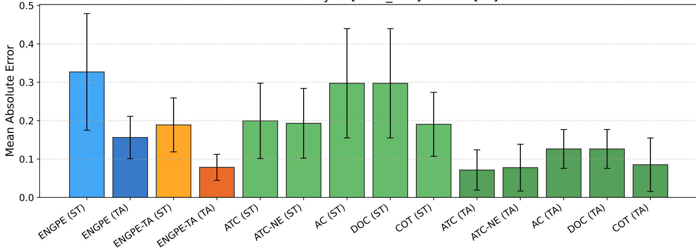
BREEDS entity30 [seed_123] — MAE [all]
