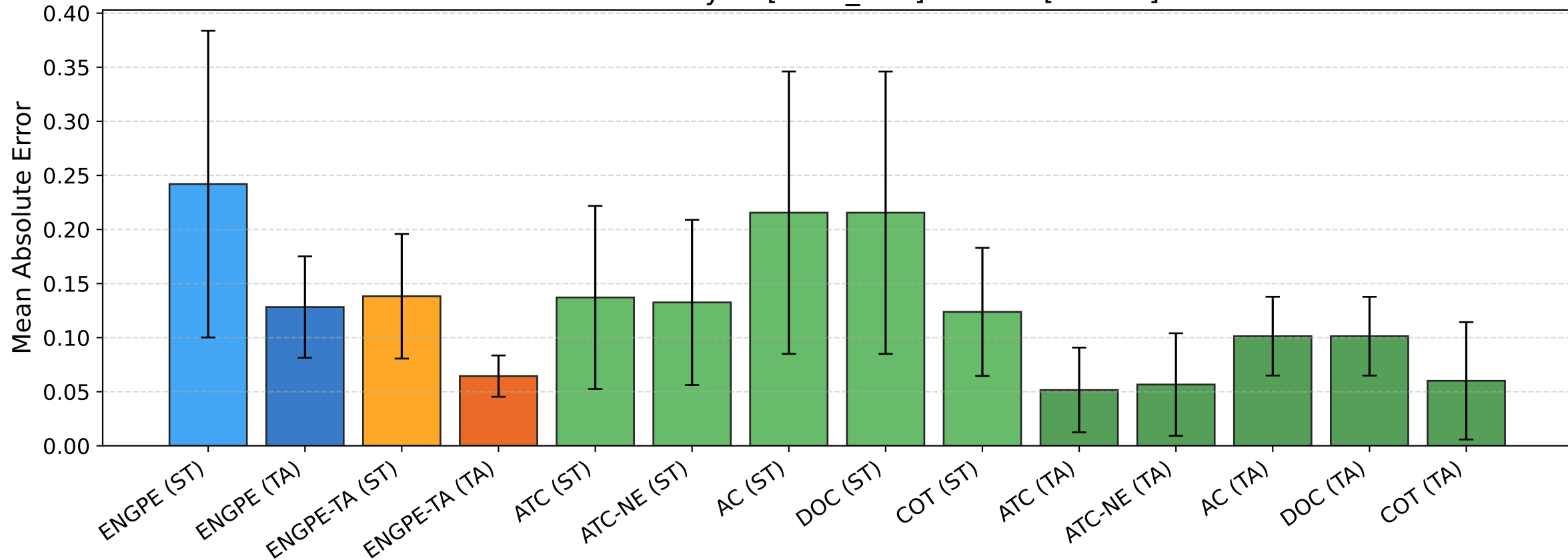
BREEDS entity30 [seed_123] — MAE [source]
