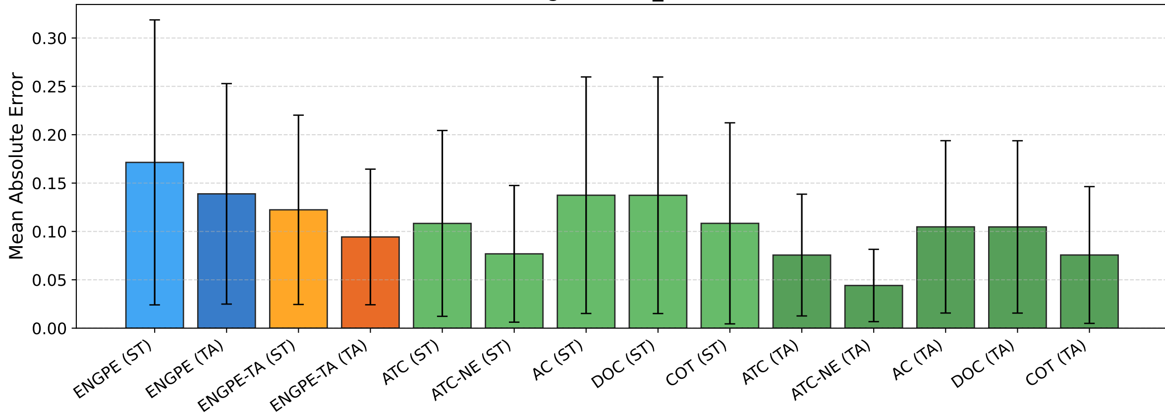
BREEDS nonliving26 [seed_123] — MAE [clean]
