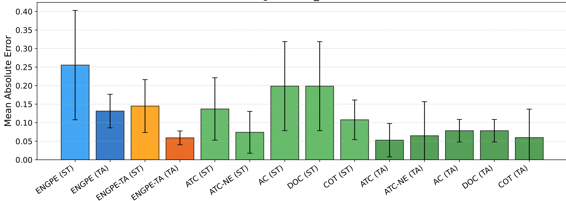
BREEDS nonliving26 [seed_123] — MAE [source]
