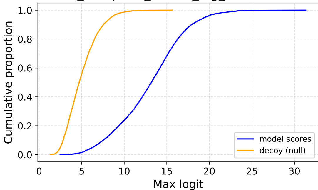
seed_123 | corr_source_fog_sev1 — ECDF
