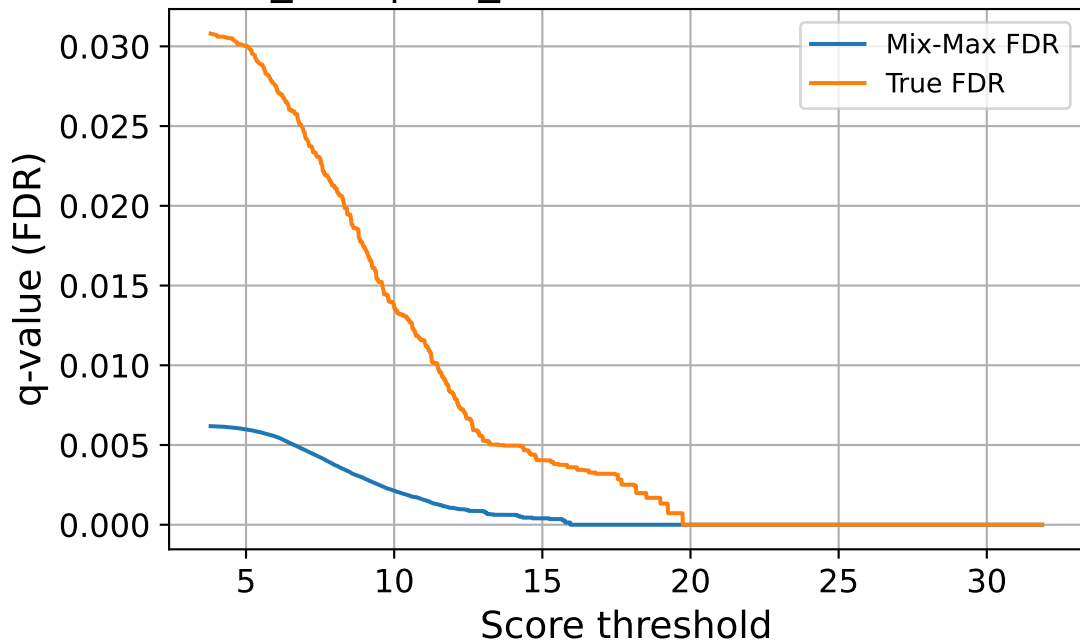
seed_123 | val_source — FDR vs Threshold
