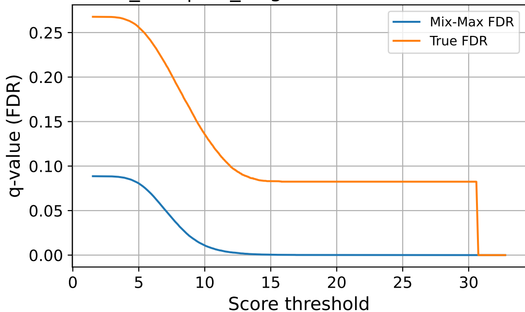
seed_123 | val_target — FDR vs Threshold
