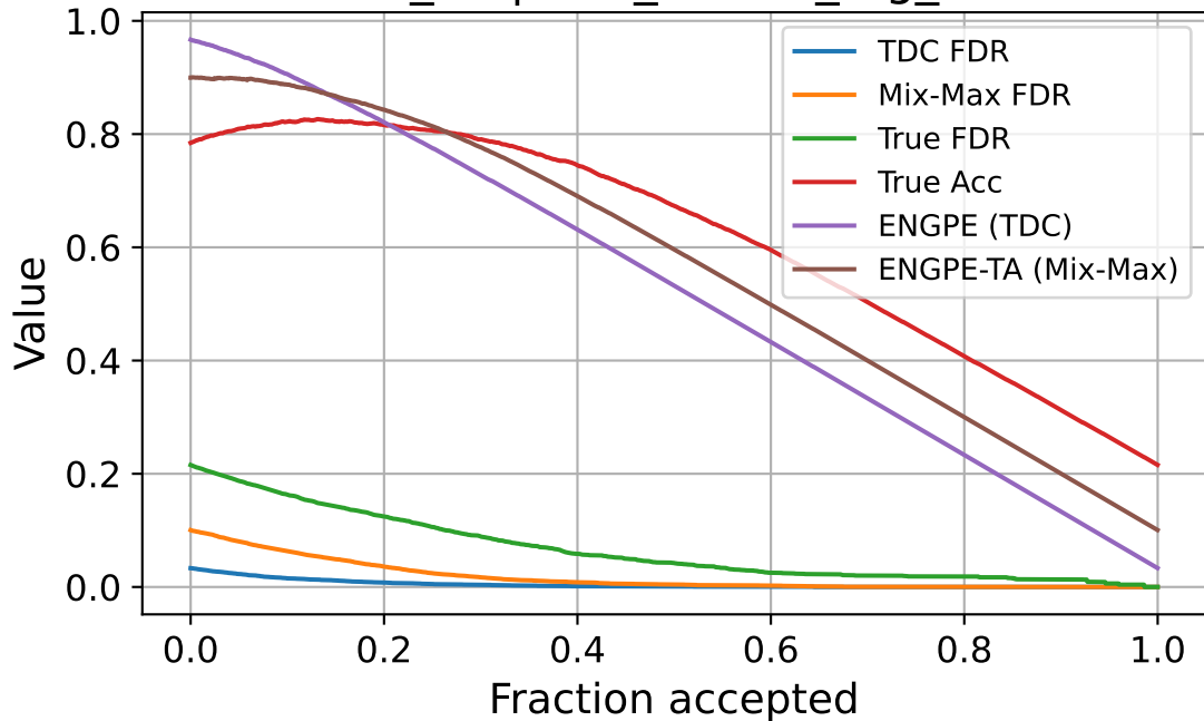
seed_42 | corr_source_fog_sev3
