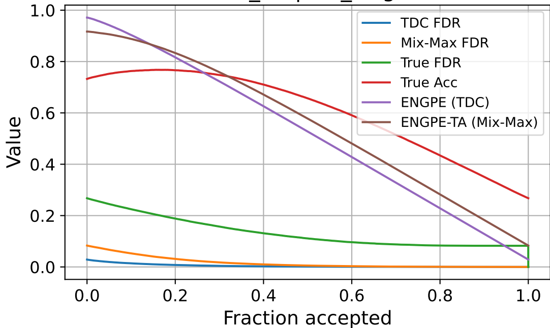
seed_42 | val_target
