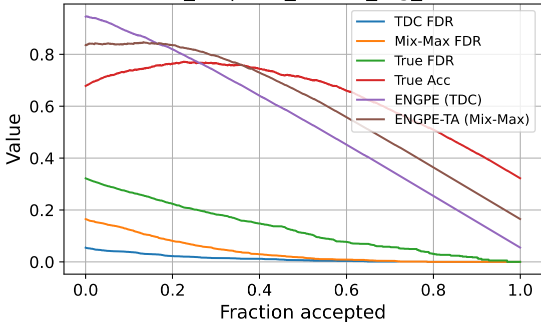
seed_42 | corr_source_fog_sev4
