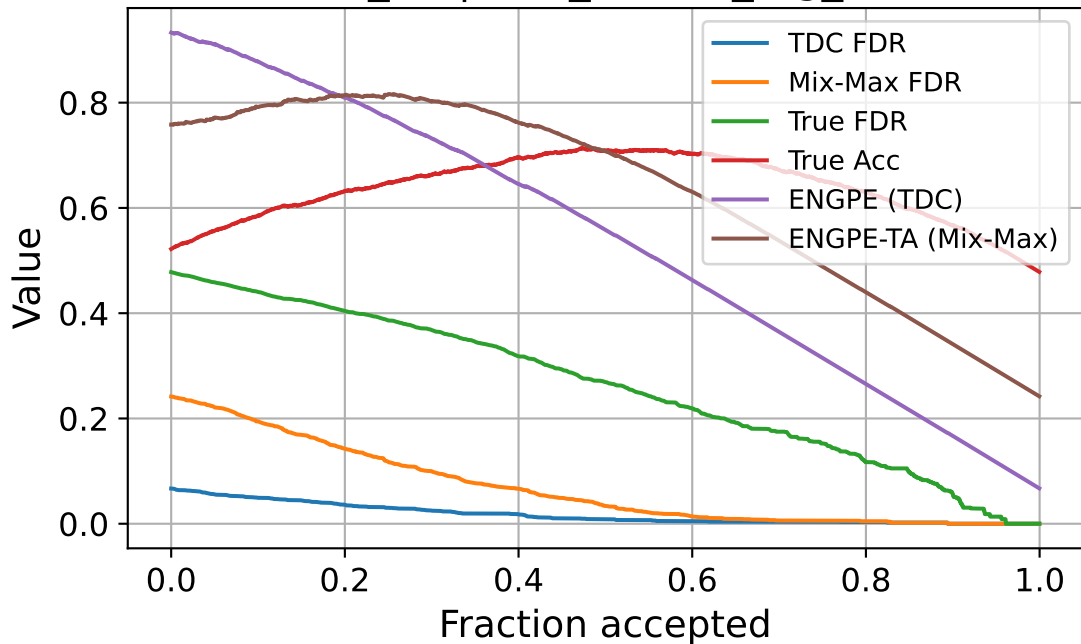
seed_42 | corr_source_fog_sev5
