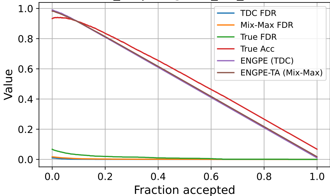
seed_42 | imagenet_val_source
