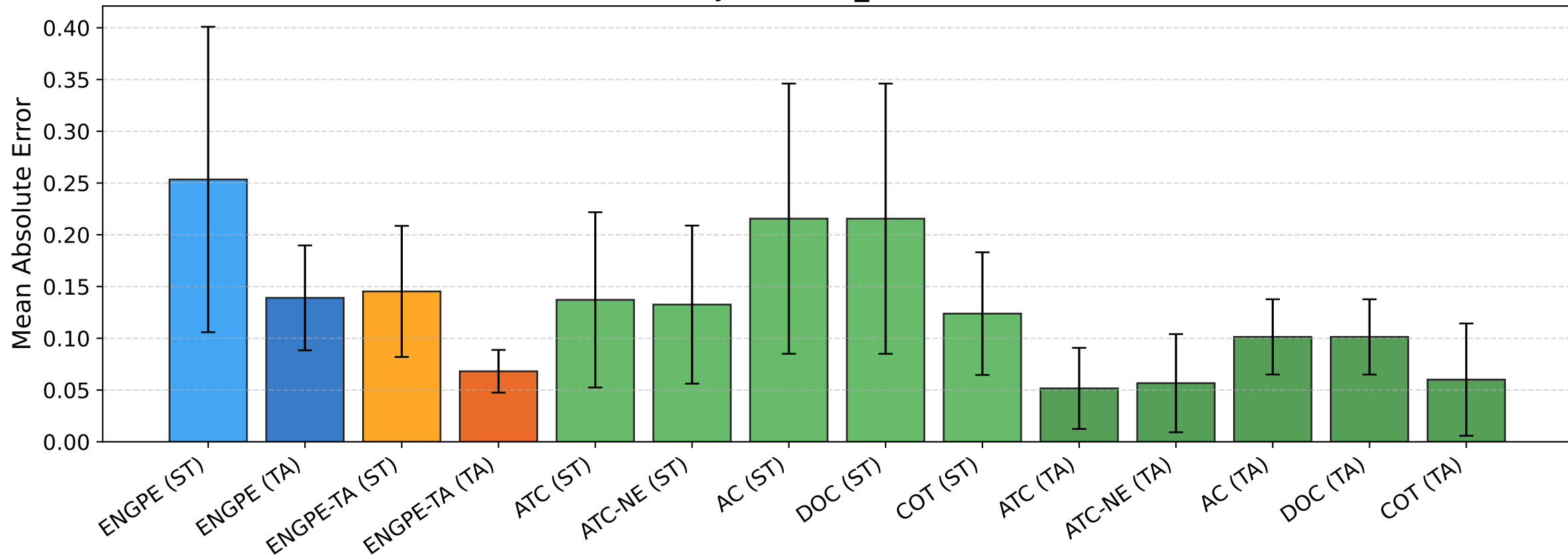
BREEDS entity30 [seed_42] — MAE [source]
