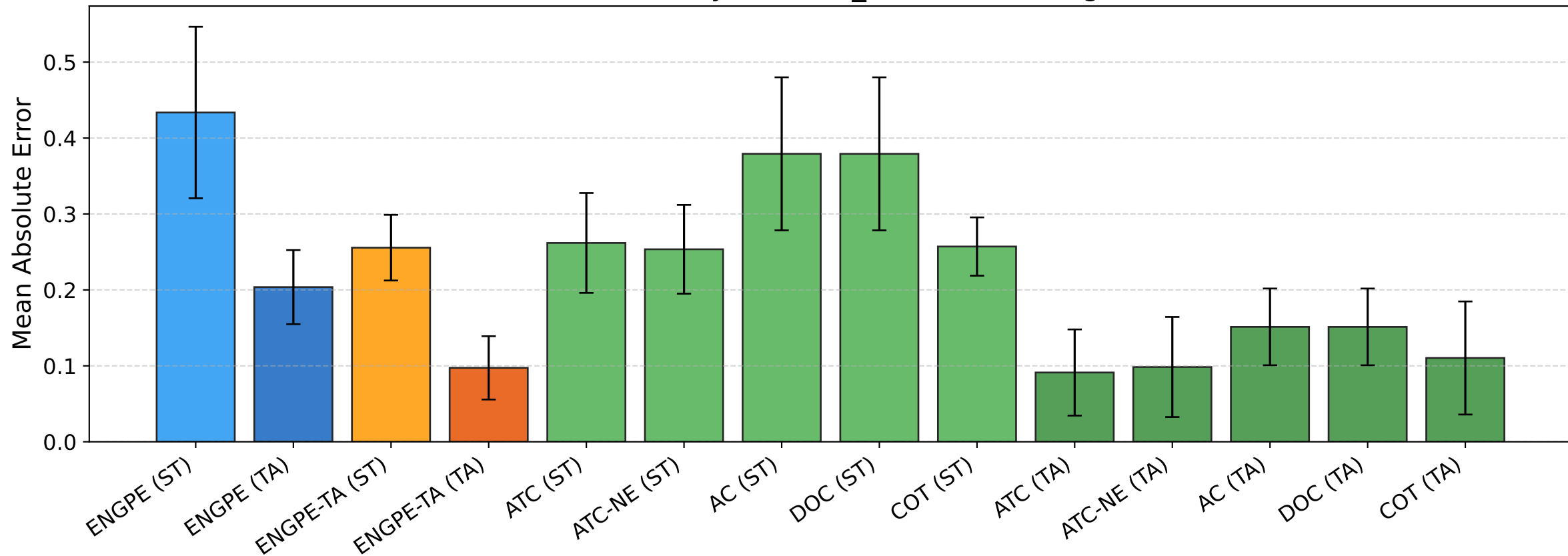
BREEDS entity30 [seed_42] — MAE [target]
