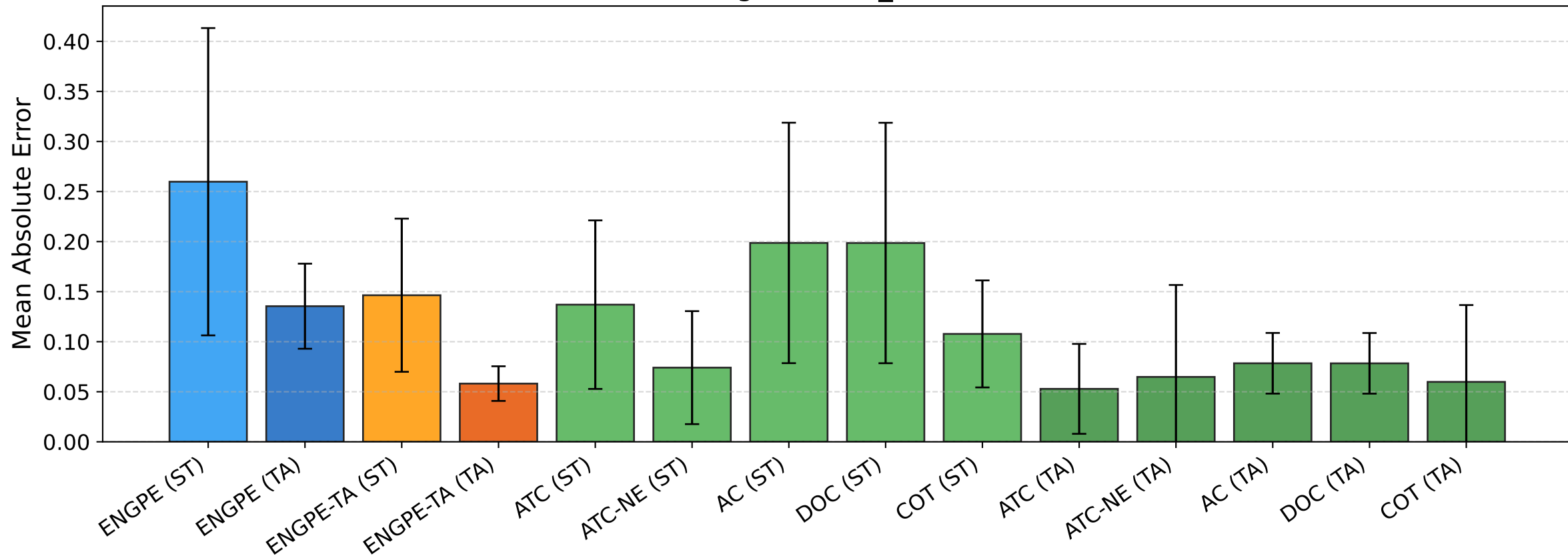
BREEDS nonliving26 [seed_42] — MAE [source]
