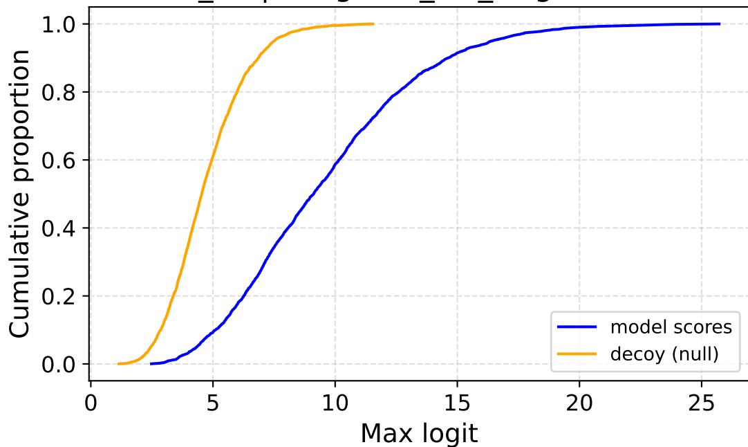
seed_42 | imagenet_val_target — ECDF
