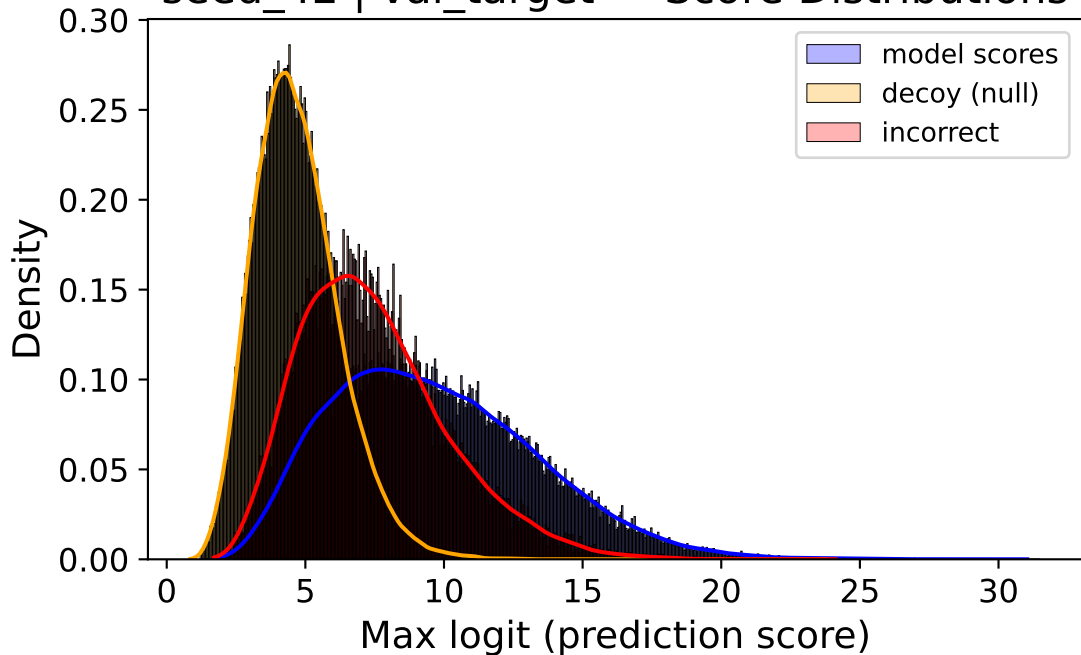
seed_42 | val_target — Score Distributions
