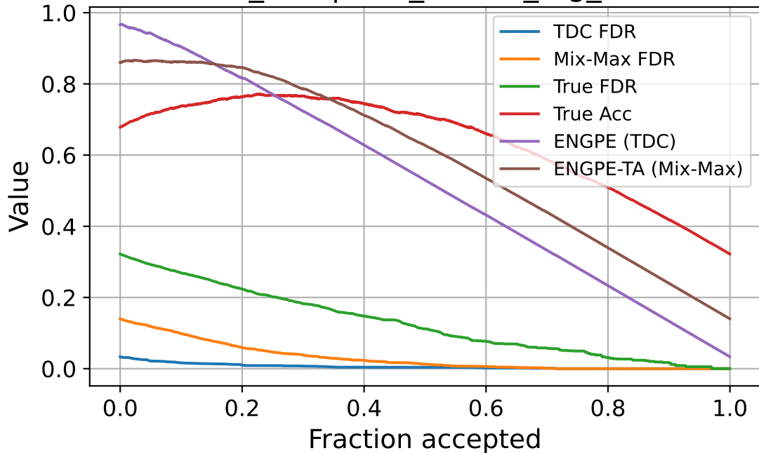
seed_456 | corr_source_fog_sev4
