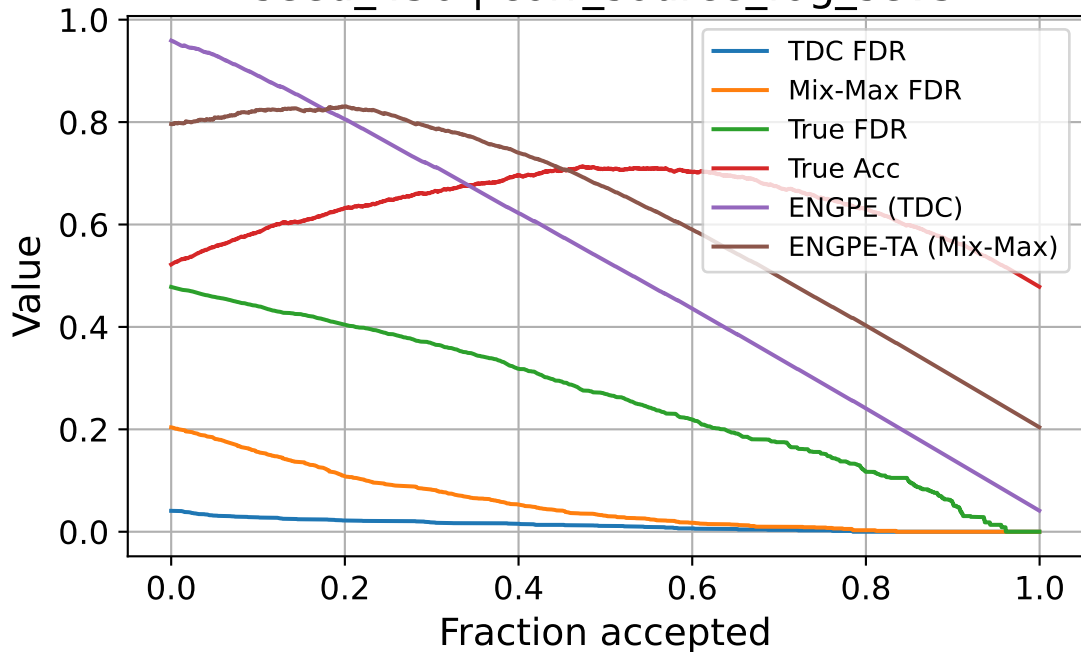
seed_456 | corr_source_fog_sev5
