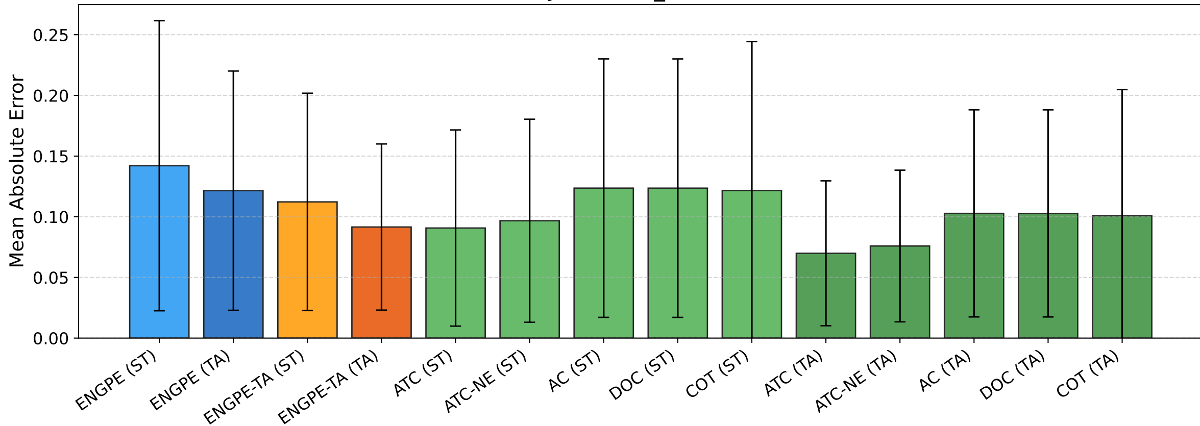
BREEDS entity30 [seed_456] — MAE [clean]
