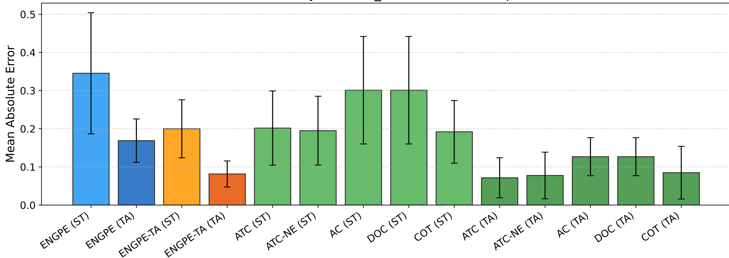
BREEDS entity30 [seed_456] — MAE [corruptions]
