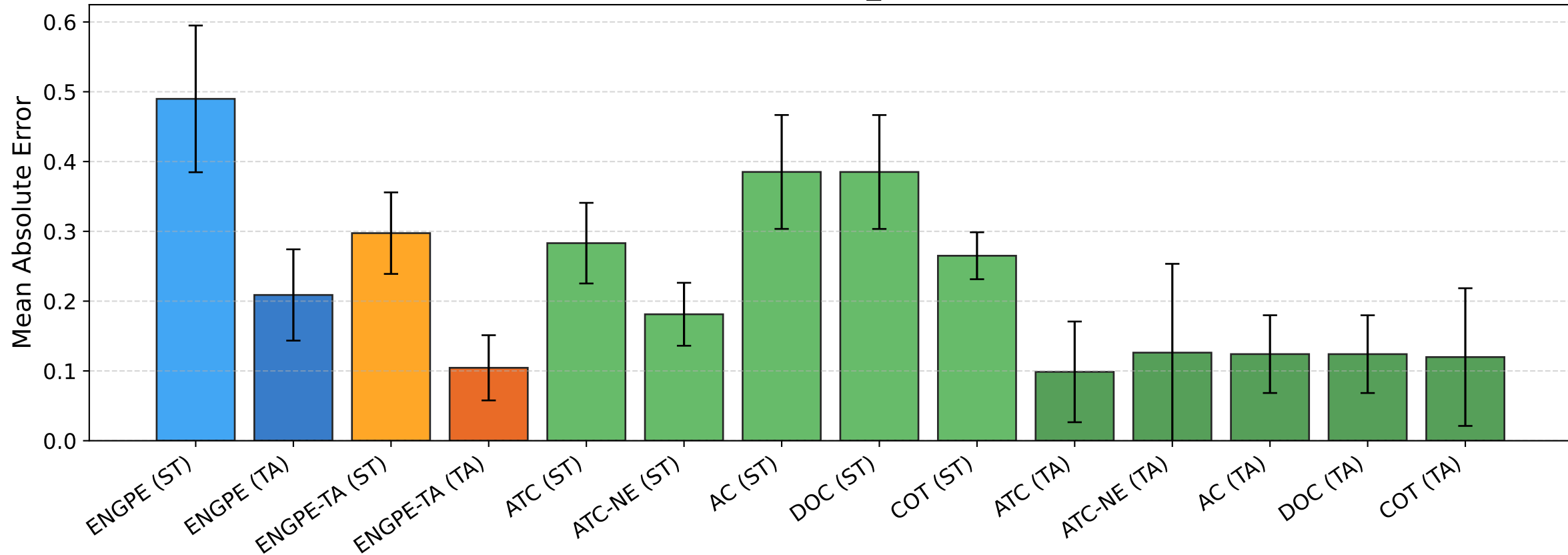
BREEDS nonliving26 [seed_456] — MAE [target]
