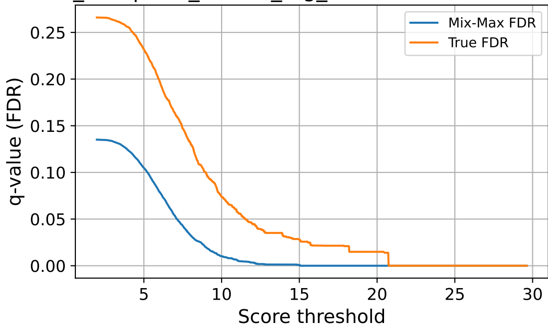
seed_456 | corr_source_fog_sev4 — FDR vs Thresh
