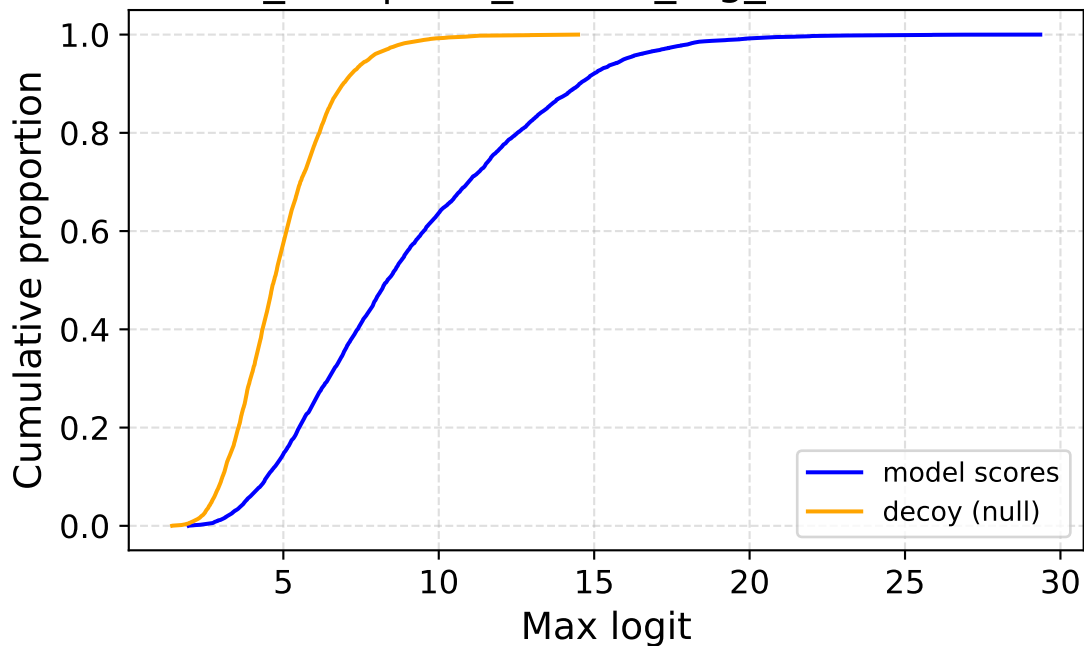
seed_456 | corr_source_fog_sev5 — ECDF
