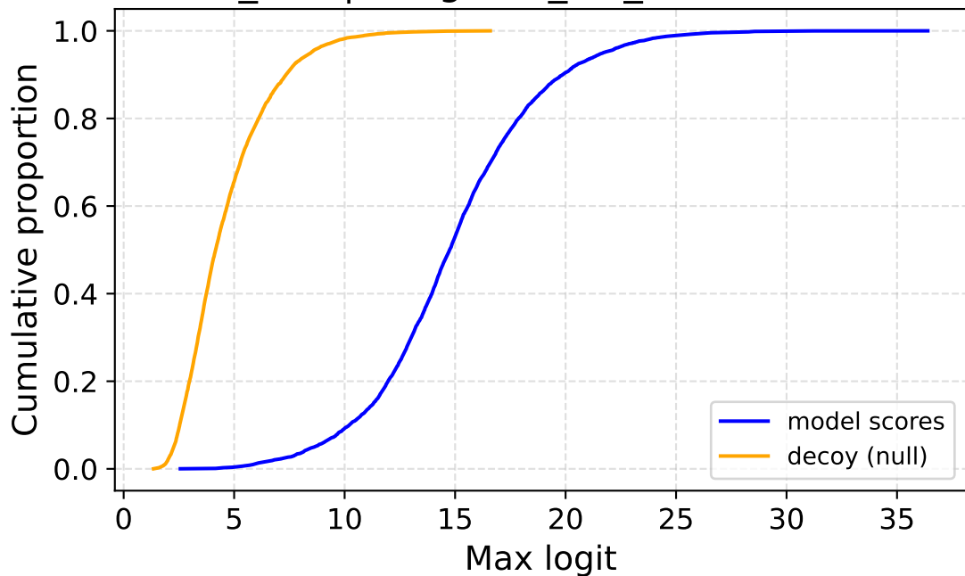
seed_456 | imagenet_val_source — ECDF
