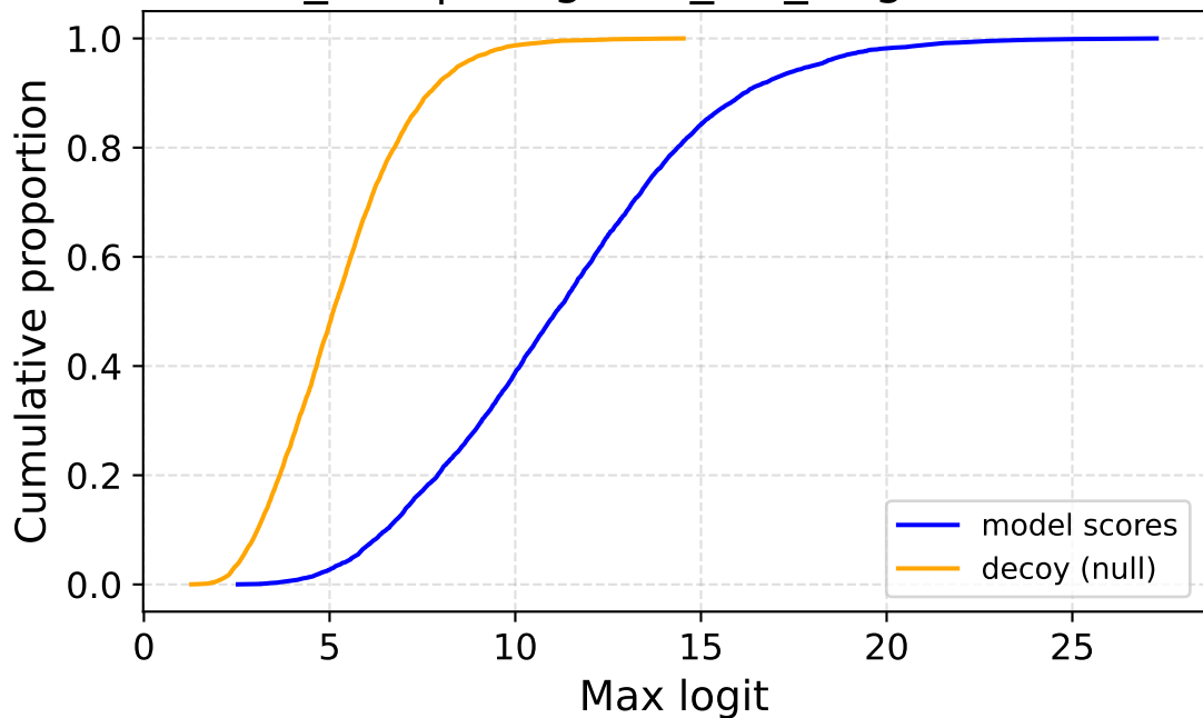
seed_456 | imagenet_val_target — ECDF
