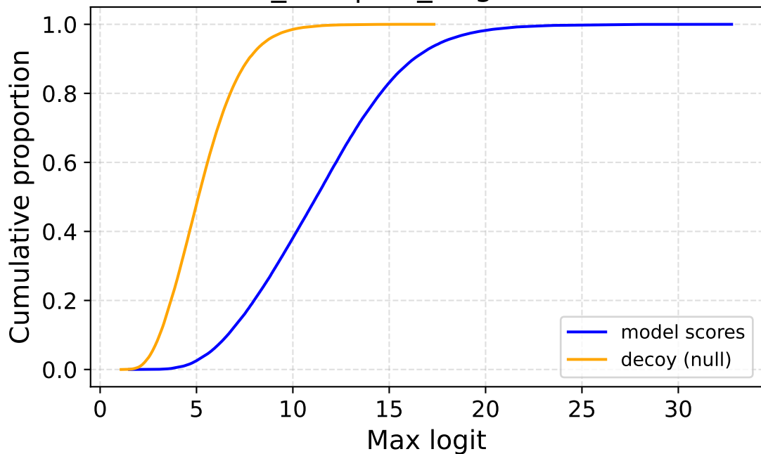
seed_456 | val_target — ECDF
