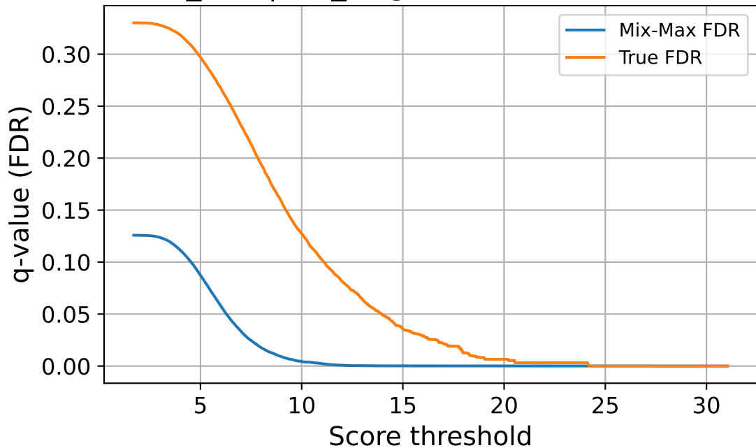
seed_456 | val_target — FDR vs Threshold
