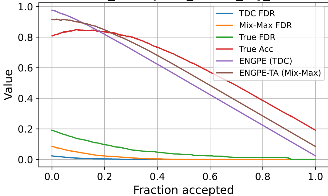
zscore_norm | corr_source_fog_sev2
