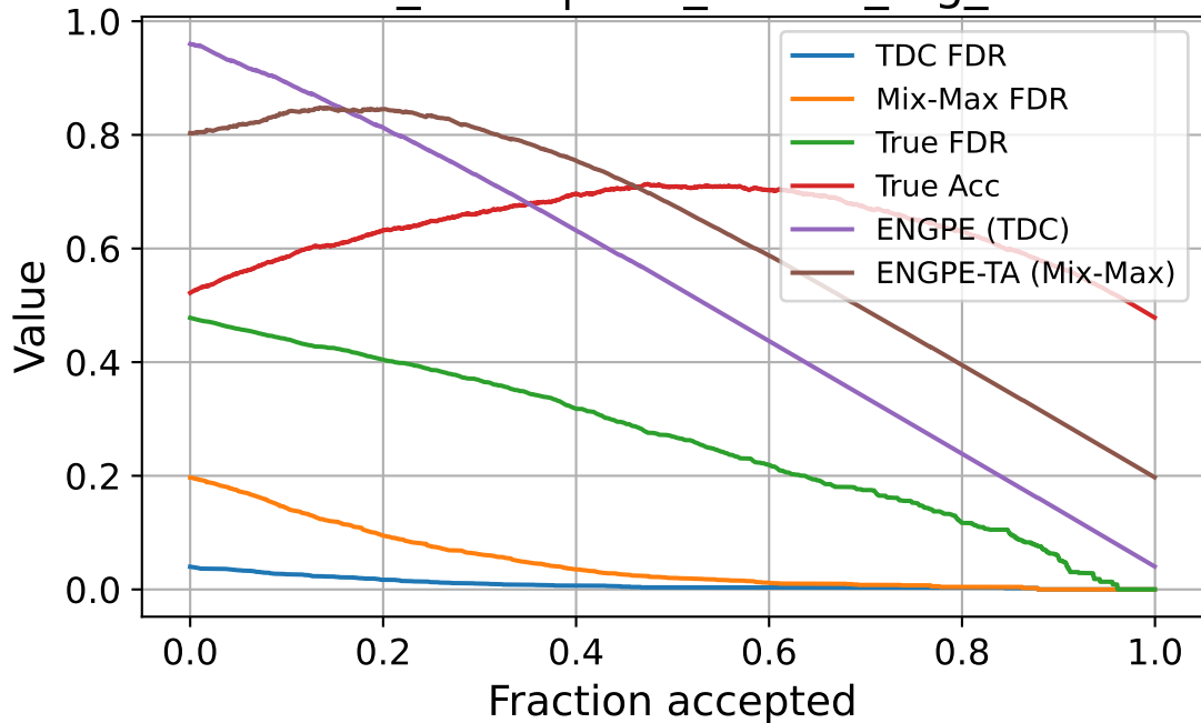
zscore_norm | corr_source_fog_sev5
