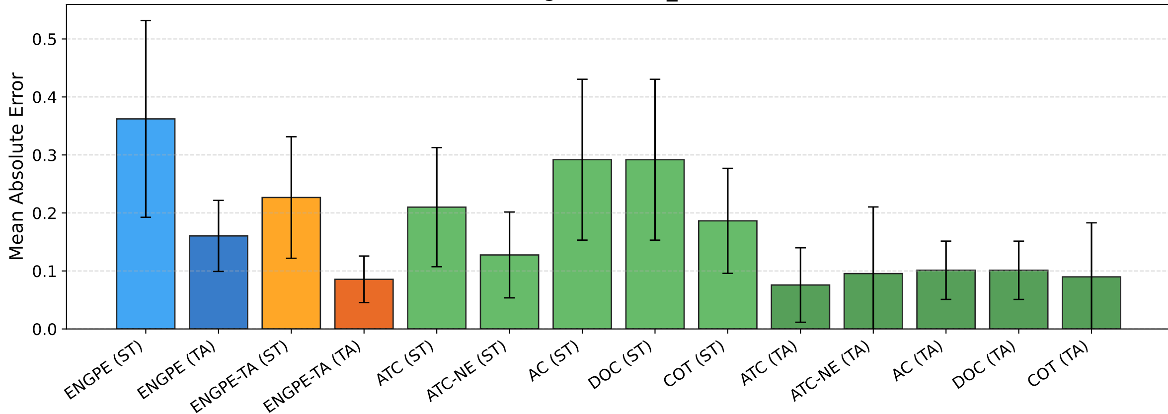
BREEDS nonliving26 [zscore_norm] — MAE [all]
