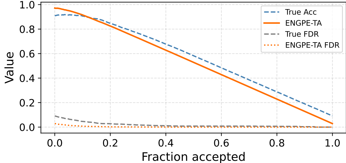
corr_source_brightness_sev1 Acc / FDR curves
