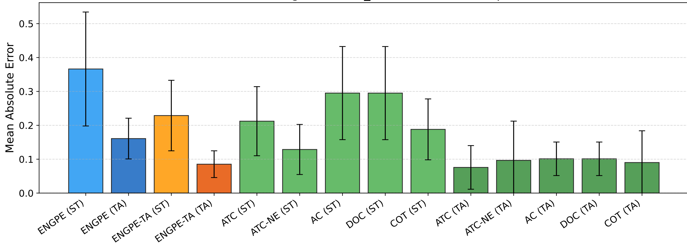
BREEDS nonliving26 [zscore_norm] — MAE [corruptions]
