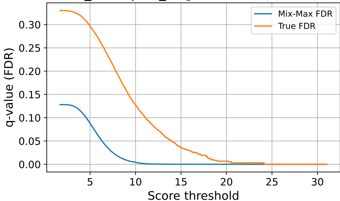
zscore_norm | val_target — FDR vs Threshold
