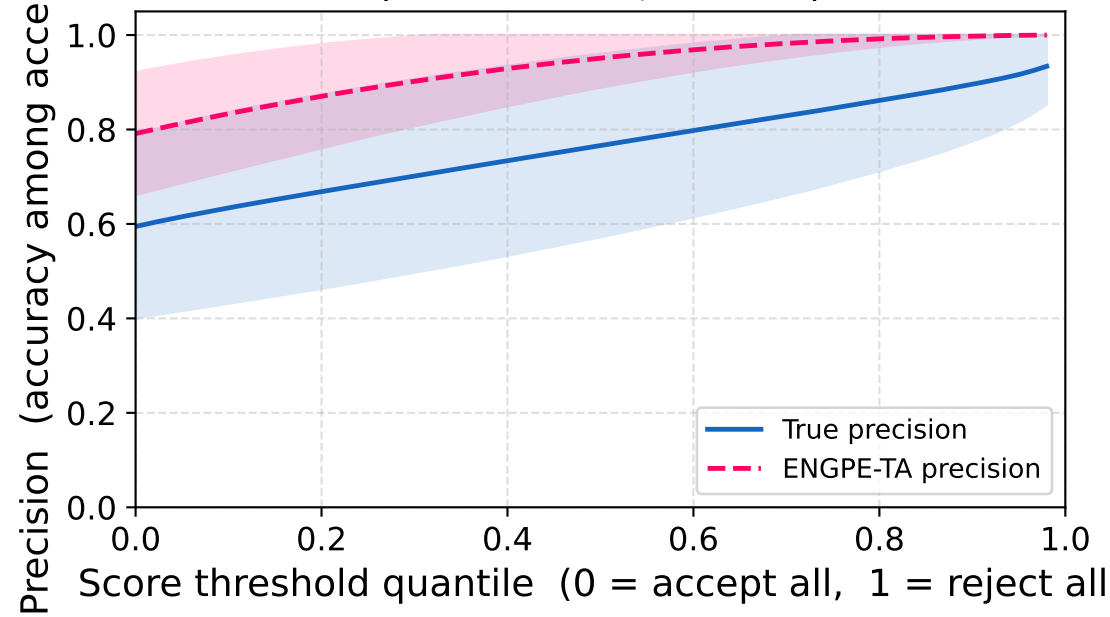
BREEDS entity30 — Precision vs Threshold (all test sets, n=194)
