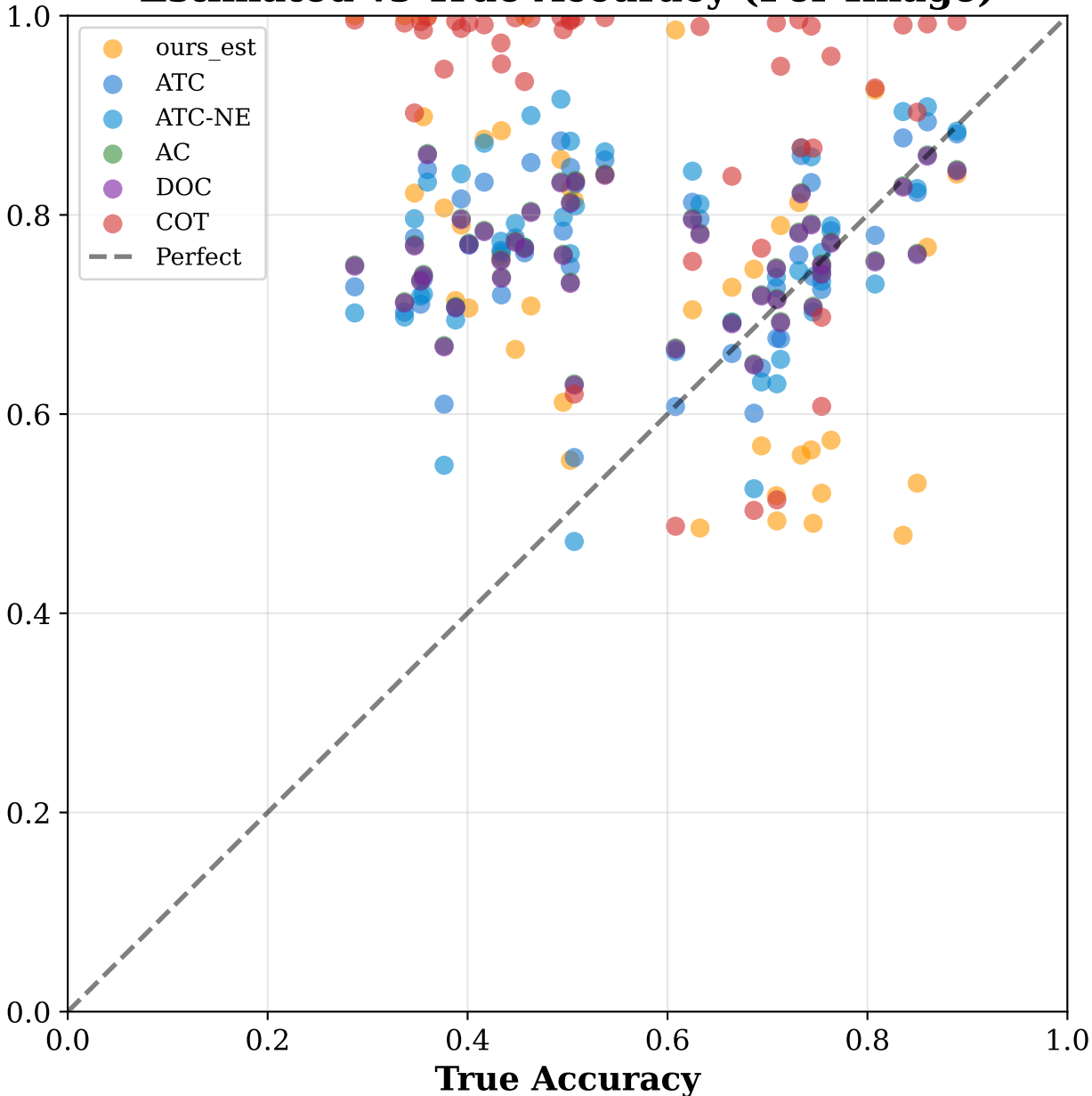
Estimated vs True Accuracy (Per Image)
