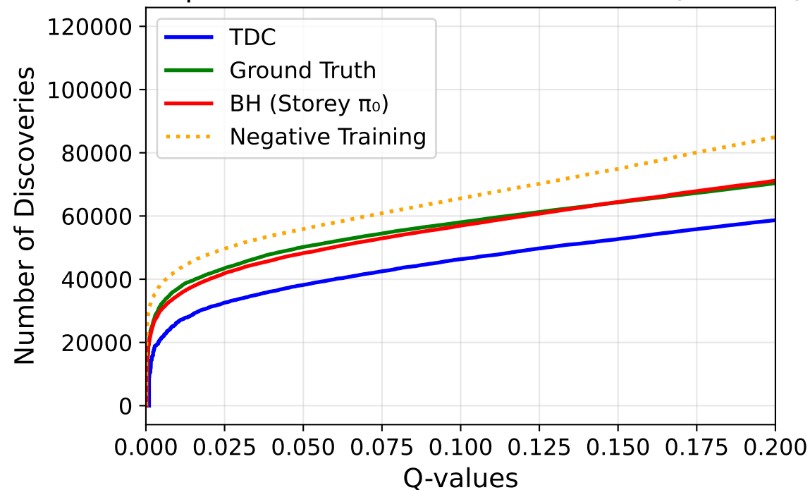
Comparison of FDR Control Methods ( \alpha \leq 0.2 )
