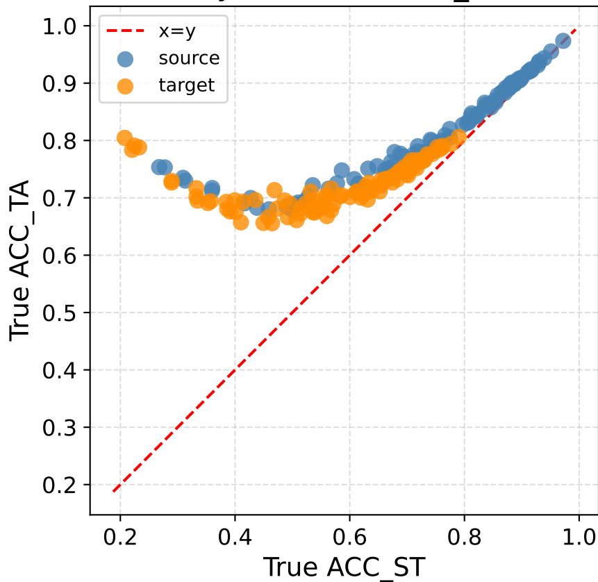
BREEDS entity13 — True ACC_ST vs ACC_TA
