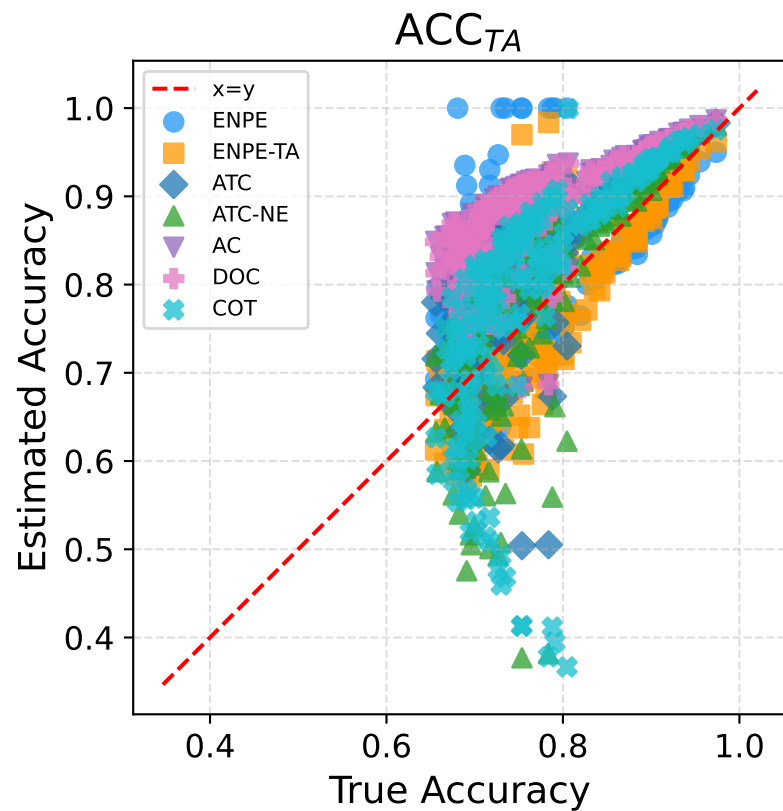
BREEDS entity13 — Estimated vs True Accuracy
