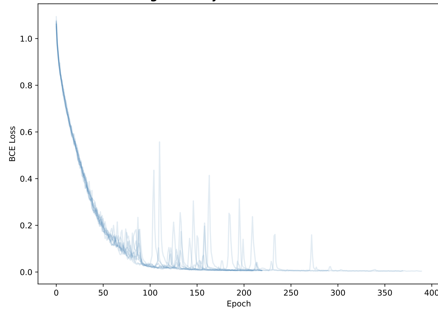
Training Loss Trajectories for Task SR-ARE
