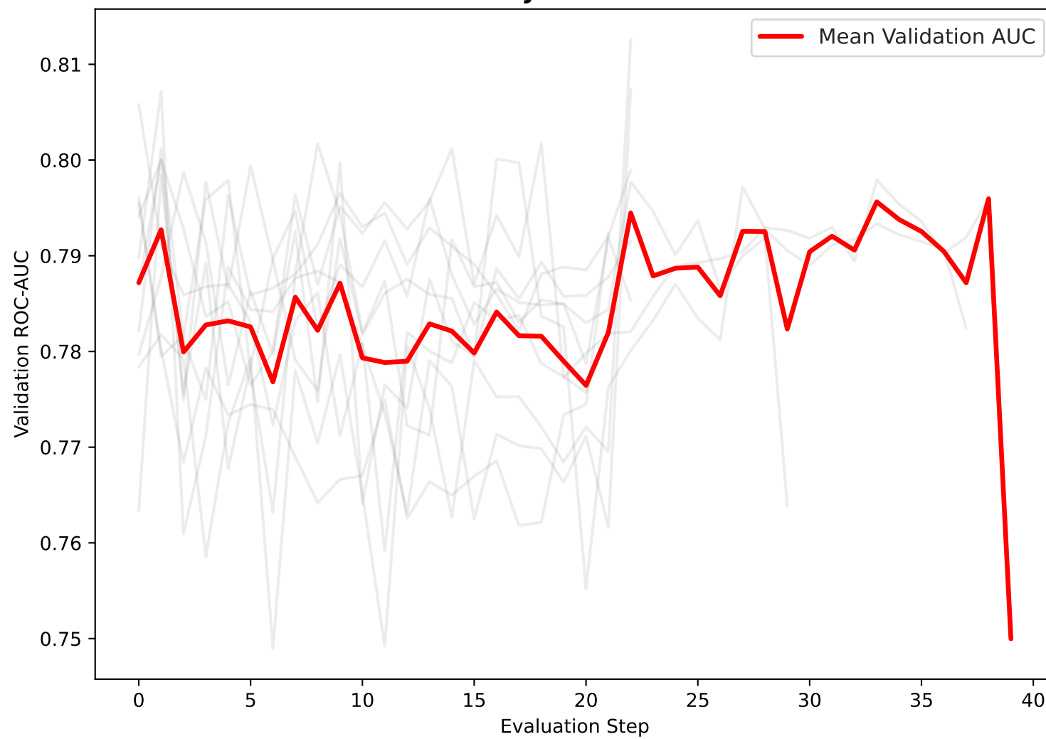
Validation AUC Trajectories for Task SR-ARE
